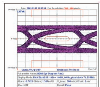
Approved Eye Pattern test for SUPRA HDMI 12m cable
